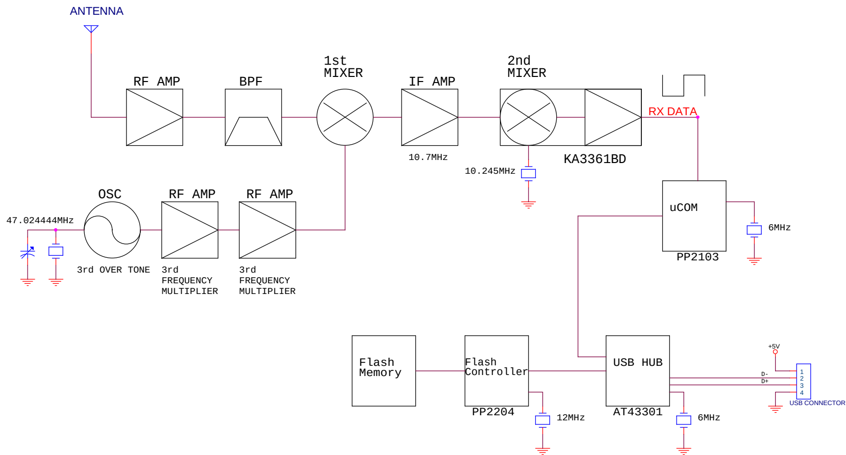
<433.92MHz RX BOARD BLOCK DIAGRAM>
