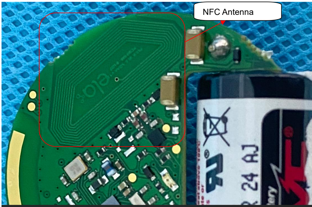
BATTERY VIEW OF EUT
