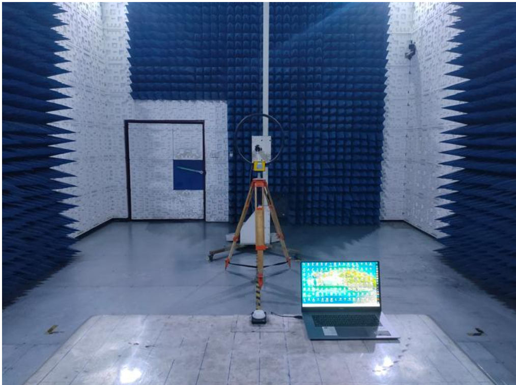
RADIATED EMISSION TEST SETUP BELOW 9KHz-30MHz
