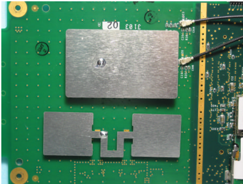
Antenna Detail, BG side
