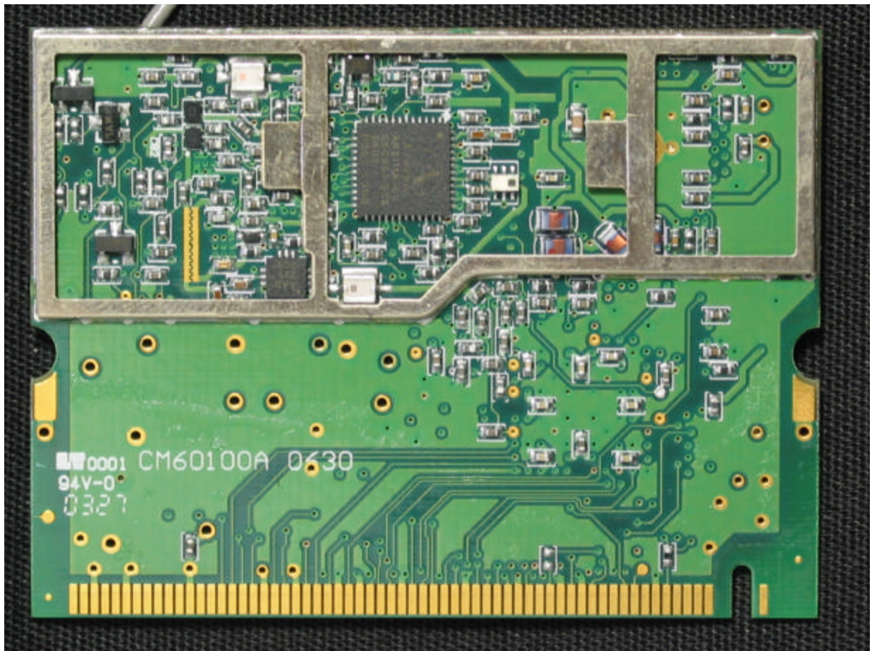
Module Detail Side 2
