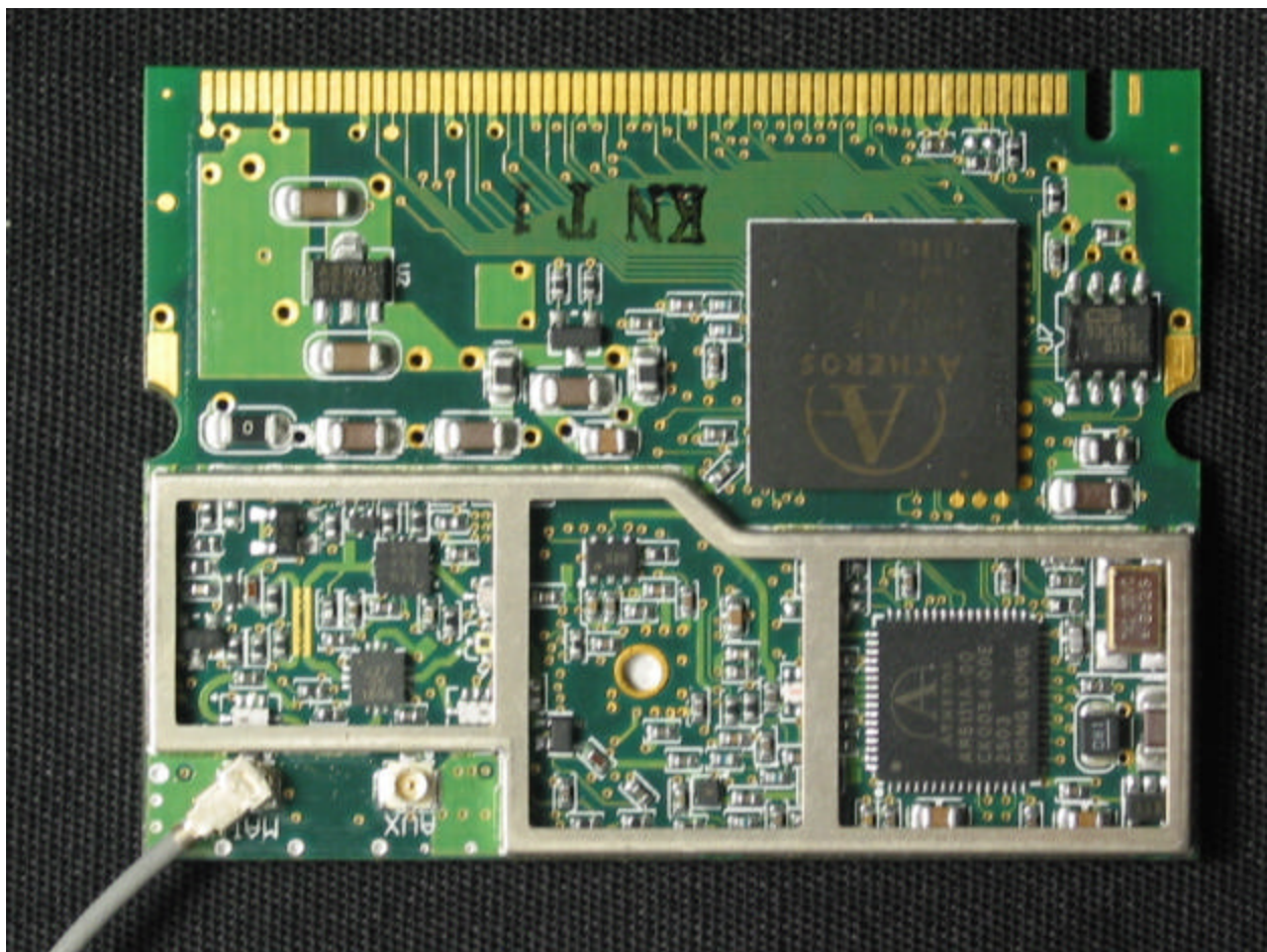
Module Detail Side 1
