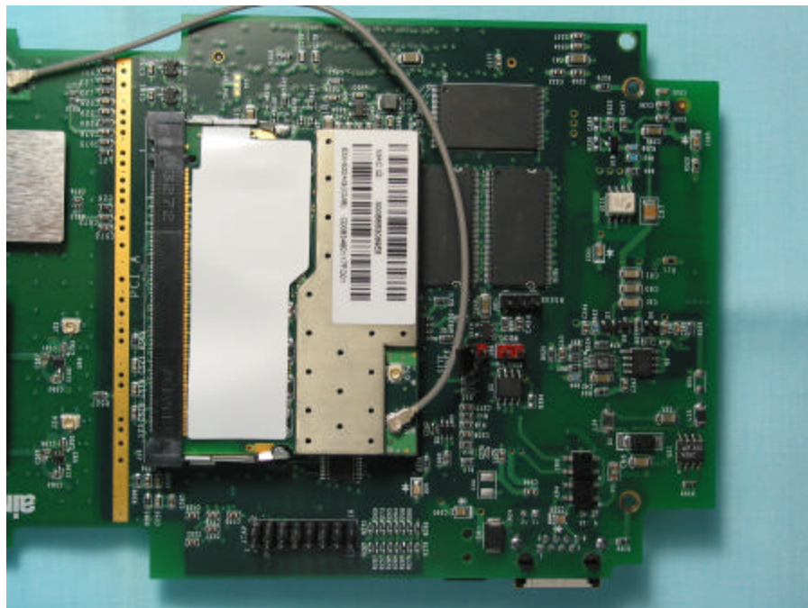
Module Detail, A Side
