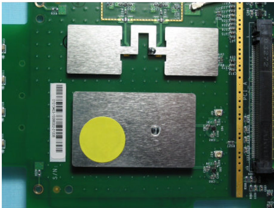
Antenna Detail, A side
