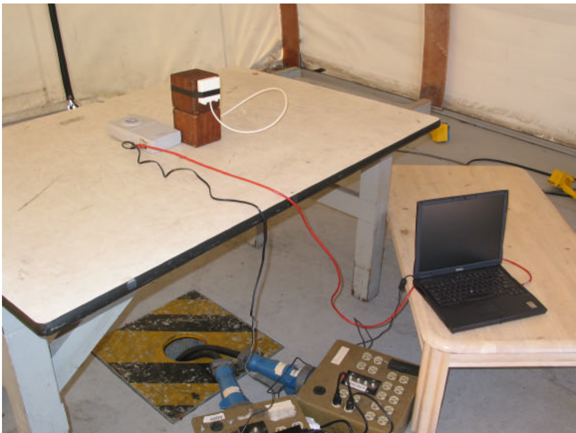
2.4 GHz Radiated emissions, external antenna
