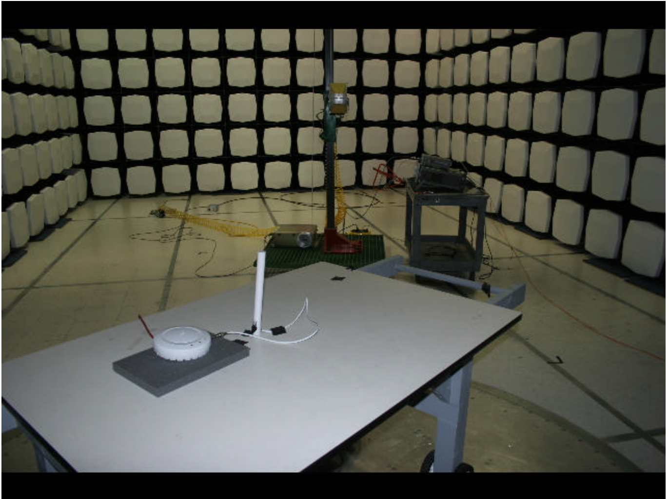
Radiated Emissions, 5.15 dBi Omni, 2.4 GHz Antenna
