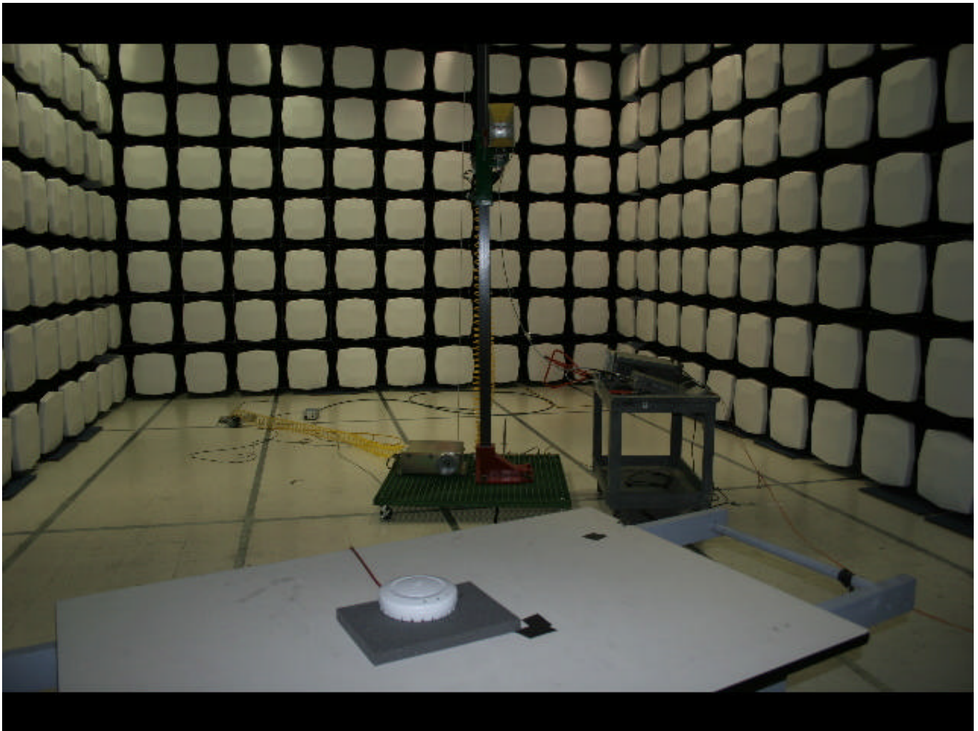
Radiated Emissions, Internal Antenna
