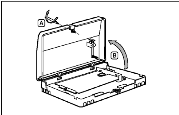
Fig. 1 : Opening housing
