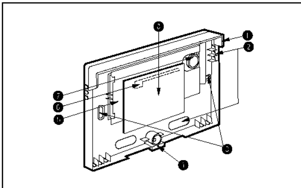
Fig. 2 : Product overview
