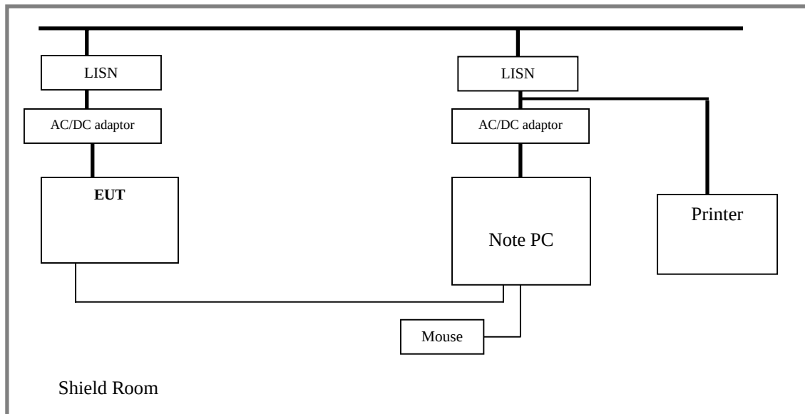
Continuous Disturbance Voltage, Main Terminal
