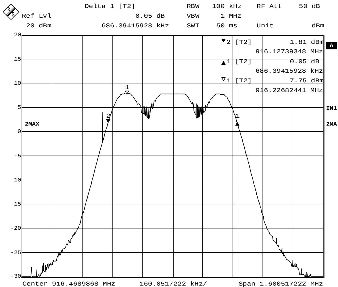
Figure 7 - 6dB Bandwidth, 686.39kHz
