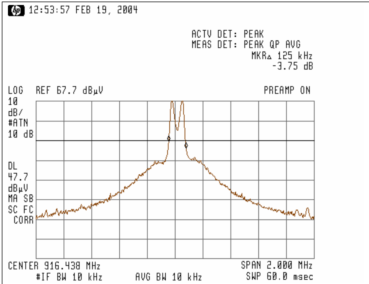
Graph # 3-3-2 20dB Occupied Bandwidth
