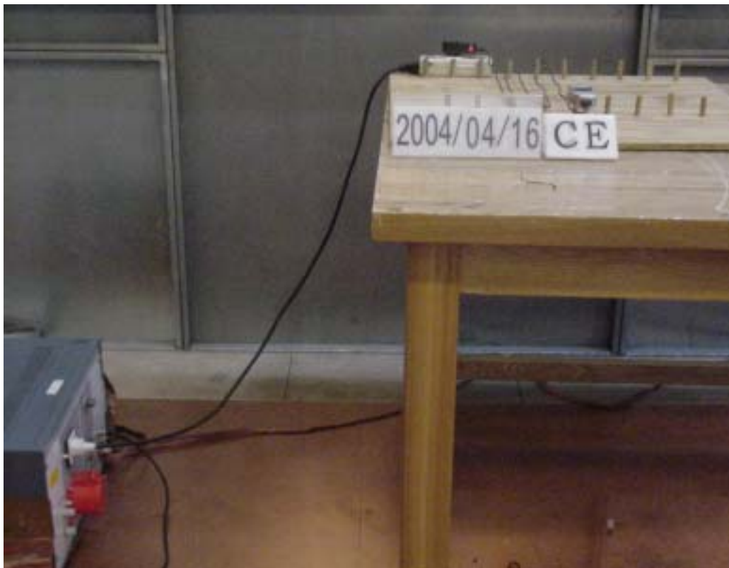
Pic1 Conducted Emission
