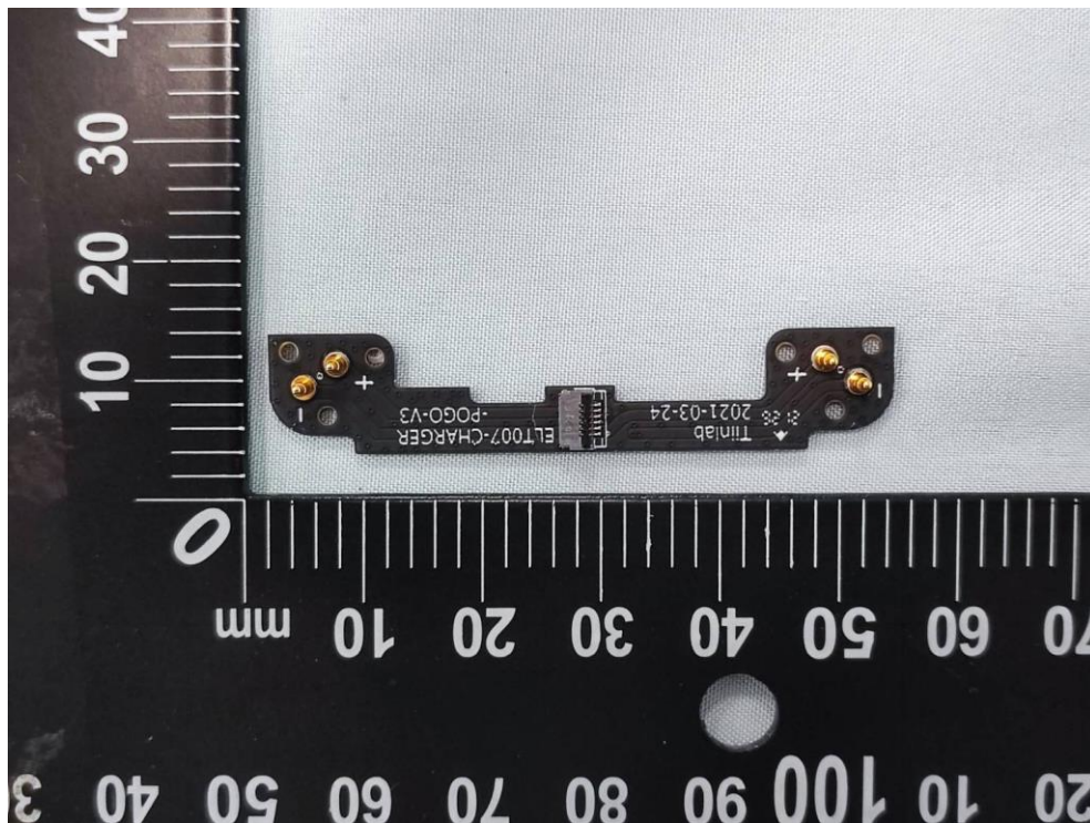
(20) EUT Photo_Chargeing Case
