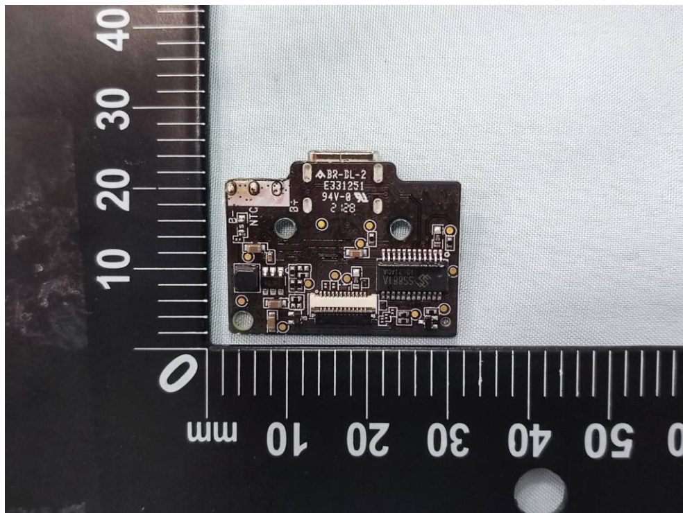
(22) EUT Photo_Chargeing Case
