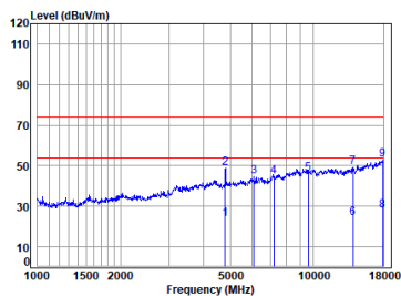
Right BT_DH5_TX_CH_00_Horizontal
