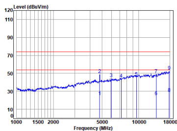
Right BT_DH5_TX_CH_00_Vertical
