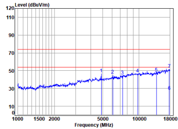
Right BT_DH5_TX_CH_39_Vertical
