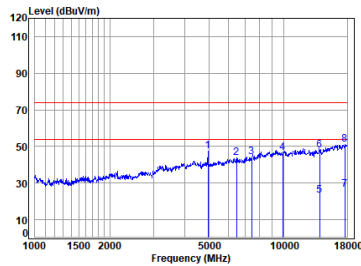
Right BT_DH5_TX_CH_78_Horizontal
