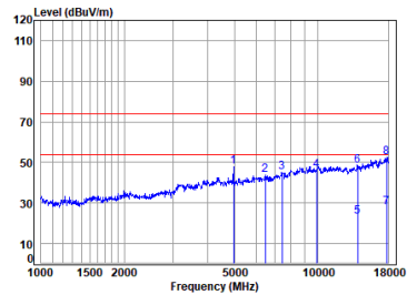
Right BT_DH5_TX_CH_78_Vertical
