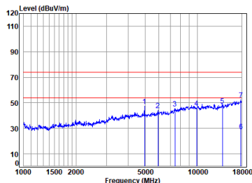
Left BT_DH5_TX_CH_78_Vertical
