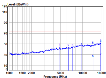
Left BT_DH5_TX_CH_39_Vertical
