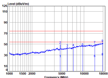
Left BT_DH5_TX_CH_00_Vertical
