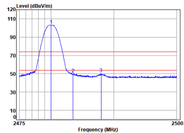
Left BT_DH5_TX_CH_78_Vertical
