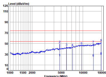
Left BT_DH5_TX_CH_00_Horizontal
