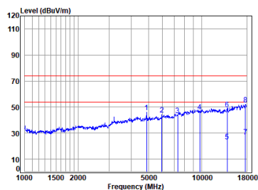
Left BT_DH5_TX_CH_39_Horizontal
