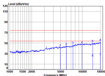
2.4G SRD_1M_TX_CH_39_Vertical-Peak
