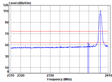
2.4G SRD_1M_TX_CH_00_Horizontal-Peak
