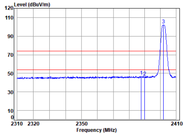
2.4G SRD_2M_TX_CH_00_Vertical-Peak
