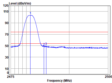
2.4G SRD_1M_TX_CH_39_Horizontal-Peak
