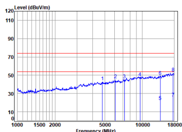
2.4G SRD_2M_TX_CH_00_Horizontal-Peak
