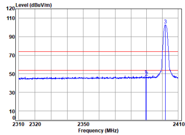
2.4G SRD_1M_TX_CH_00_Vertical-Peak
