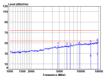
2.4G SRD_1M_TX_CH_00_Horizontal-Peak
