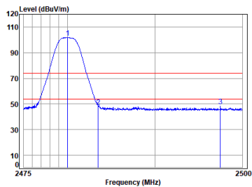
2.4G SRD_2M_TX_CH_39_Vertical-Peak
