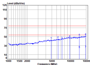
2.4G SRD_1M_TX_CH_19_Horizontal-Peak
