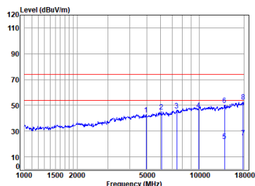
2.4G SRD_1M_TX_CH_39_Horizontal-Peak
