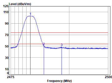
2.4G SRD_2M_TX_CH_39_Horizontal-Peak
