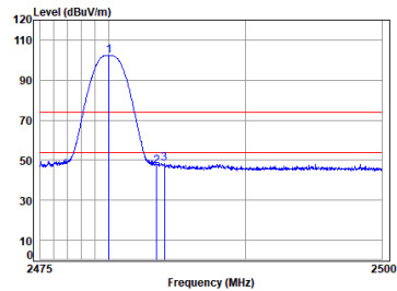
2.4G SRD_1M_TX_CH_39_Vertical-Peak
