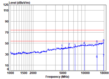
2.4G SRD_2M_TX_CH_19_Vertical-Peak
