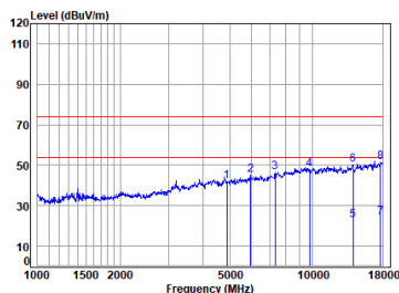
2.4G SRD_1M_TX_CH_19_Vertical-Peak
