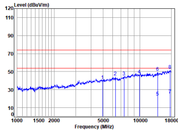
2.4G SRD_2M_TX_CH_39_Horizontal-Peak
