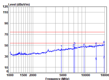
2.4G SRD_1M_TX_CH_00_Vertical-Peak
