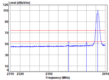
2.4G SRD_2M_TX_CH_00_Horizontal-Peak
