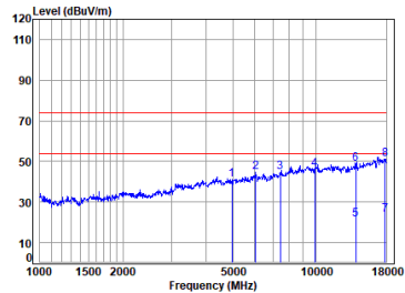
2.4G SRD_2M_TX_CH_39_Vertical-Peak
