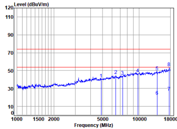
2.4G SRD_2M_TX_CH_19_Horizontal-Peak
