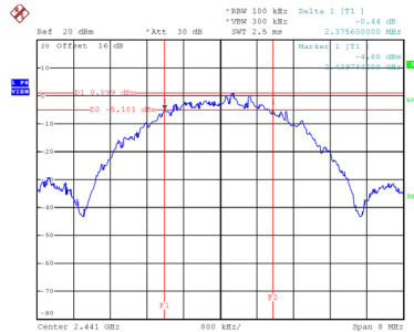
CH39 6 dB Bandwidth
