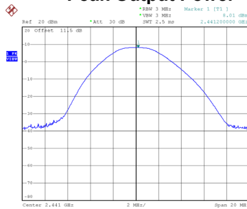
CH40 Peak Output Power
