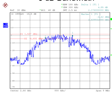
CH09 6 dB Bandwidth
