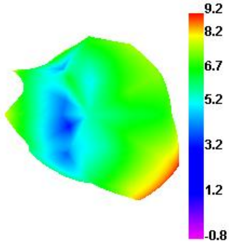
Bluetooth 39 TRP
