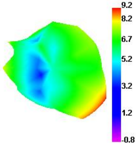
Bluetooth 39 TRP
