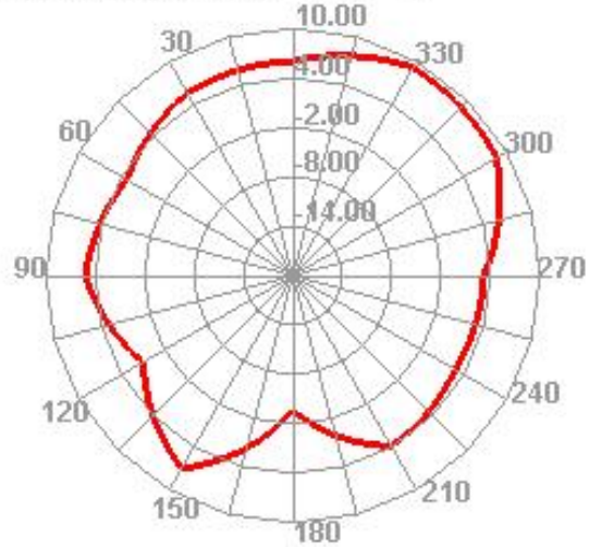
Bluetooth 39 TRP H
