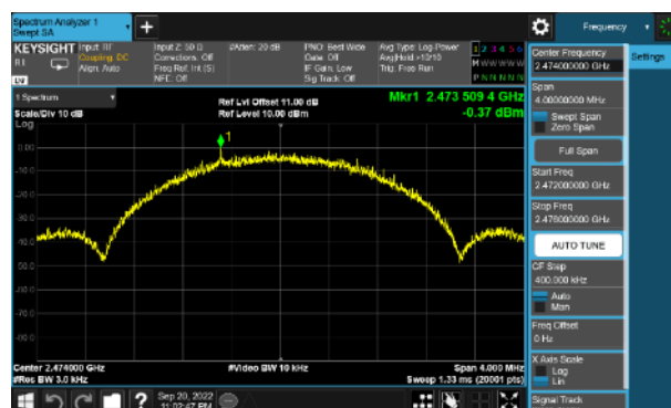
CH34 (2474MHz)
