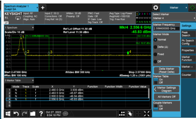
Bandedge CH79 (Upper)
