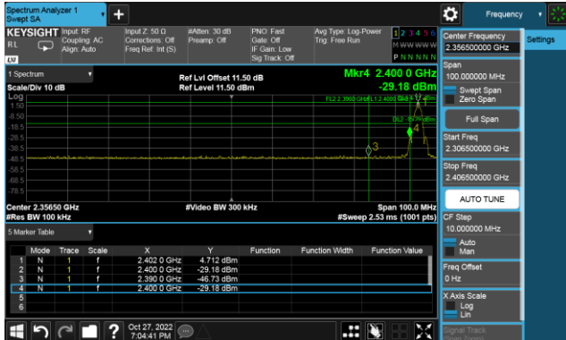
Bandedge CH01 (Lower)
