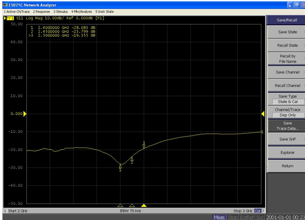
S11
