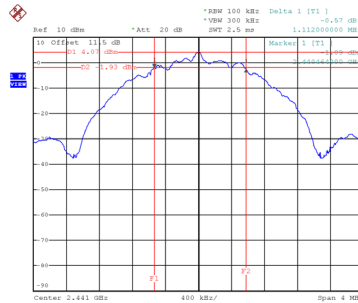
CH40 6 dB Bandwidth
