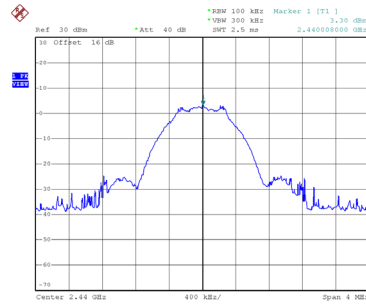
Reference Level-CH19
