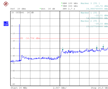
Harmonic-CH19
