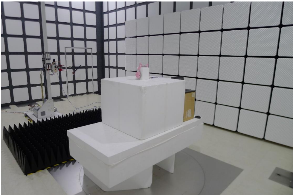
Description: Radiated Emission Test Setup for above 1GHz
