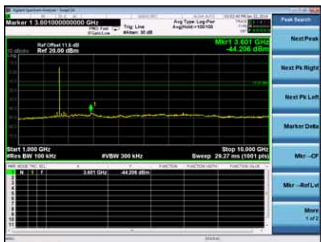
2480MHz(1GHz – 10GHz)
