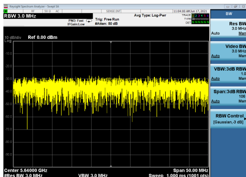
Duty Cycle_WiFi 5G
