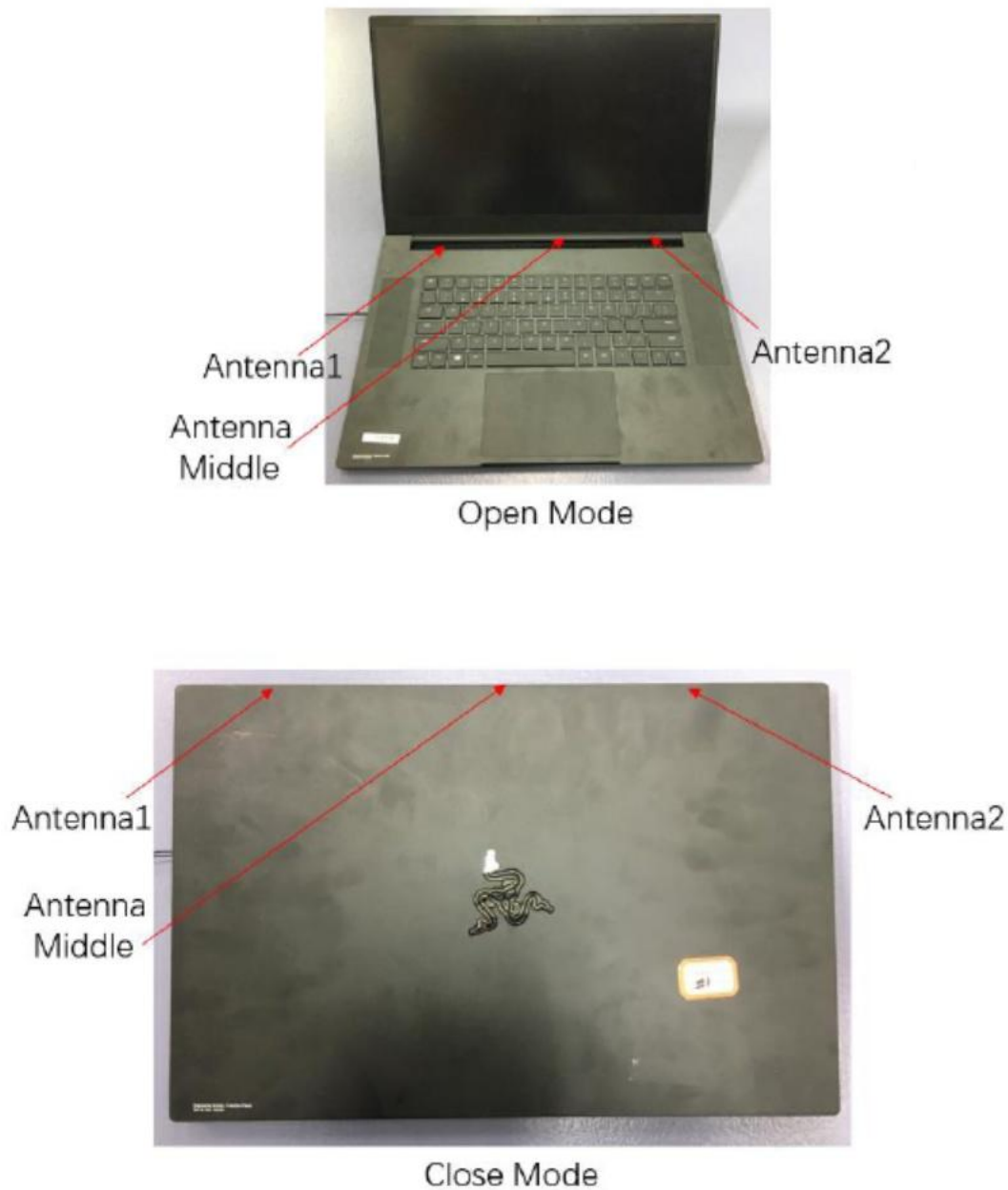
Fig.12.1 EUT Antenna Locations
