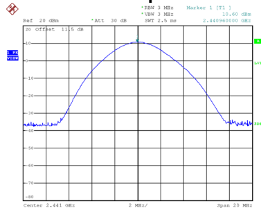
CH39 Peak Output Power
