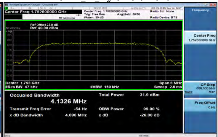
WCDMA B4 HighCH1513-1752.6
