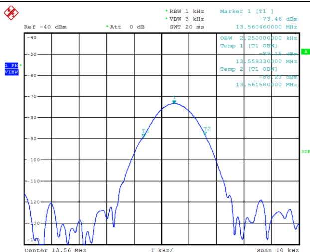
Emission Bandwidth Plot - 99% Bandwidth
