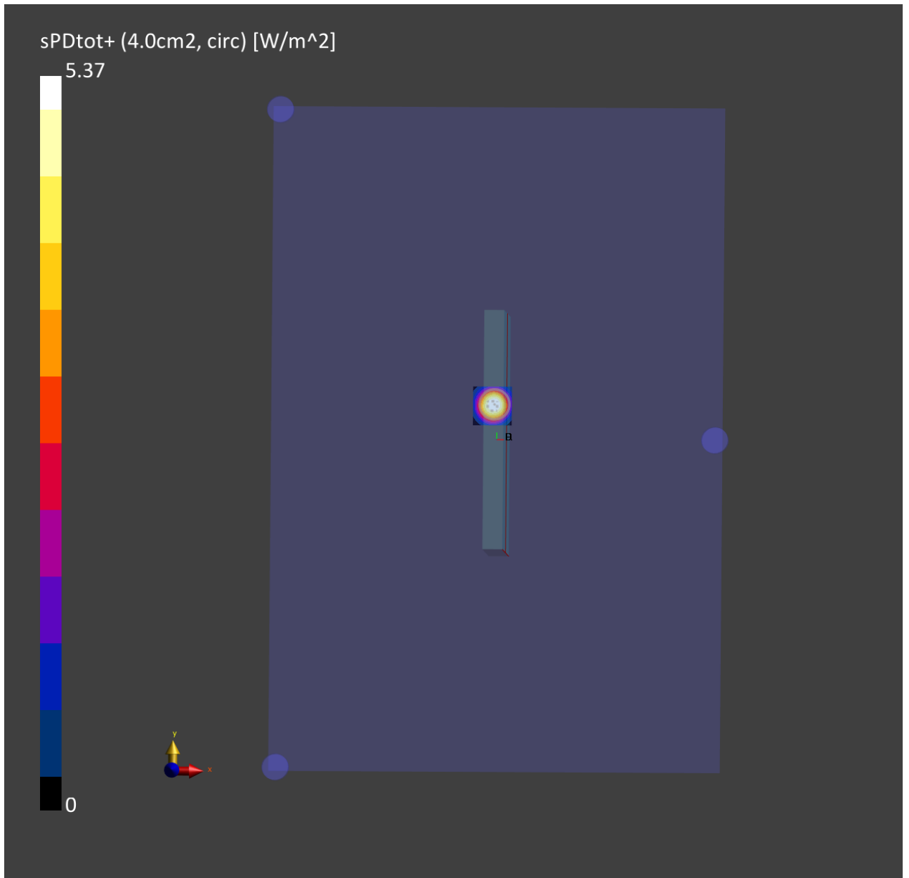
Figure 9-3: 4cm 2 -averaged power density distribution measured at input.power.limit of 9.4dBm on the back surface for n260 beam 2
