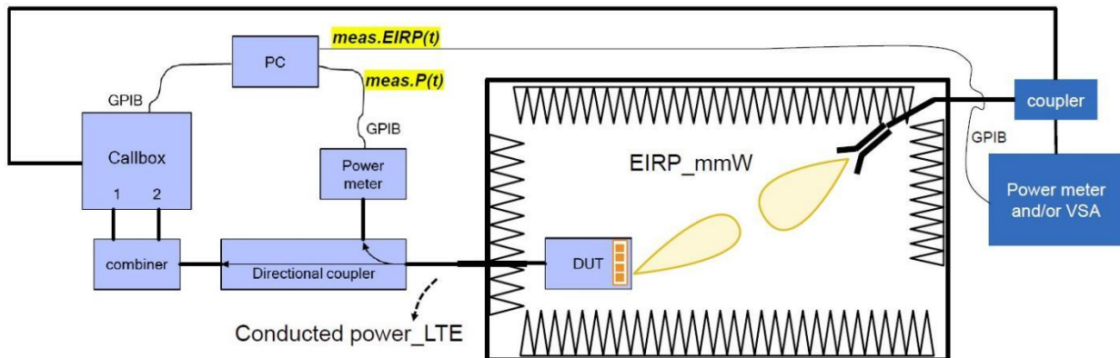
Figure 9-1 mmW NR radiated power measurement setup
