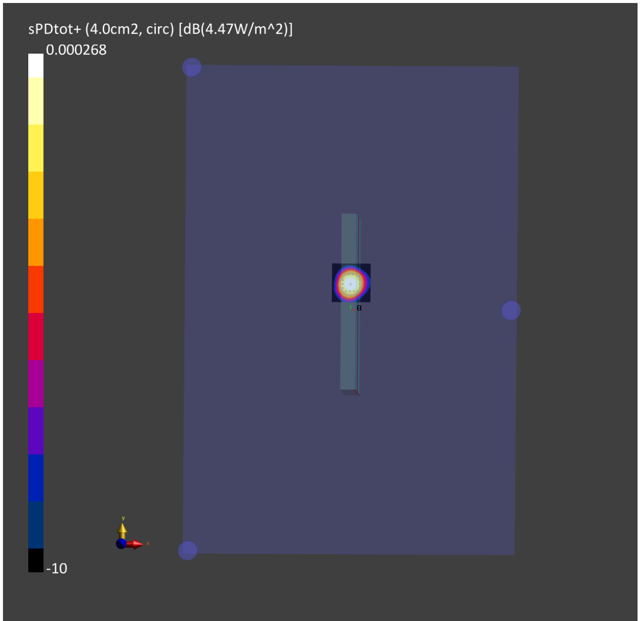
Figure 9-4: 4cm2-averaged power density distribution measured at input.power.limit of 4.1dBm on the back surface for n261 beam 24
