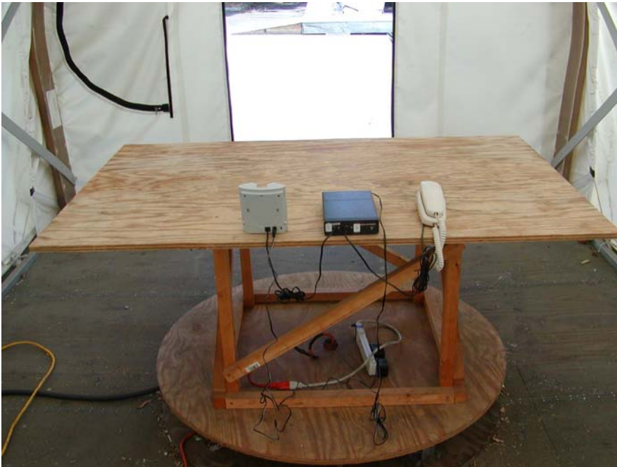
Base Radiated Emission - Rear View
