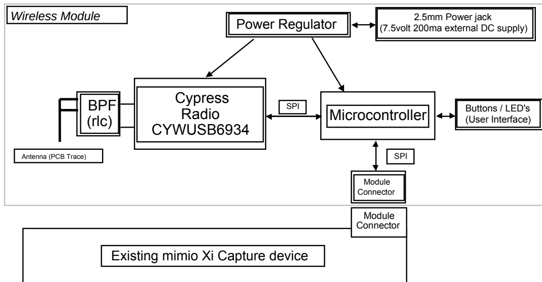
Figure 2: Wireless device module with attached mimio Xi capture device.
