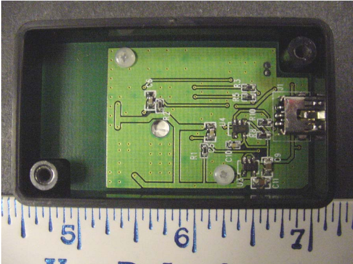
Interior of EUT with cover removed, Top of PCB
