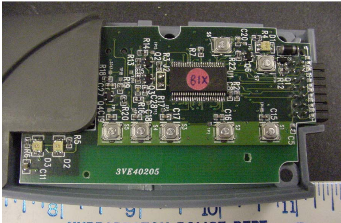
Top of PCB with cover of RF module removed.
