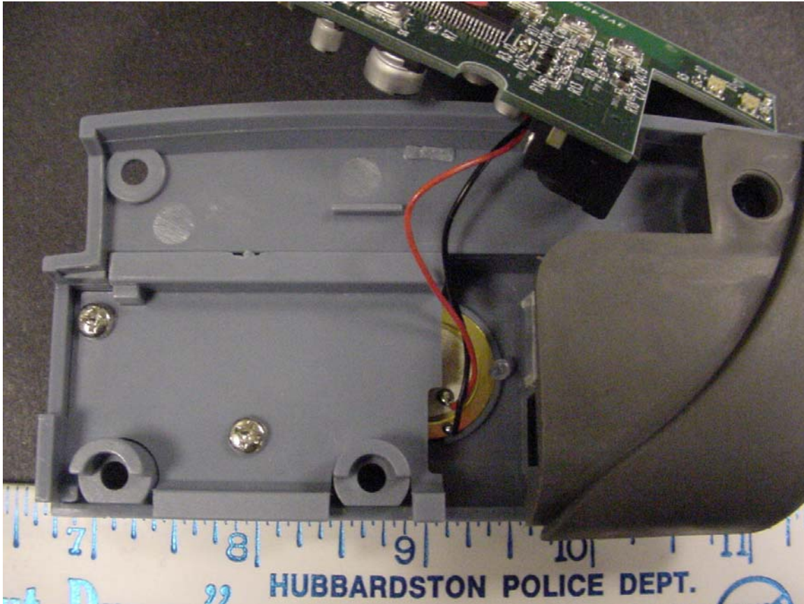
Interior of EUT with cover removed and PCB moved to the side, shows the speaker and connecting wires.
