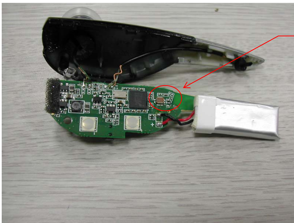
Connection to the antenna
