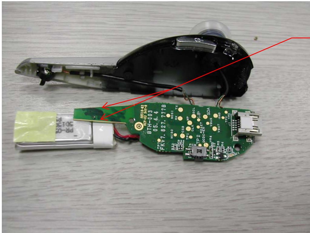
Microstrip Antenna
