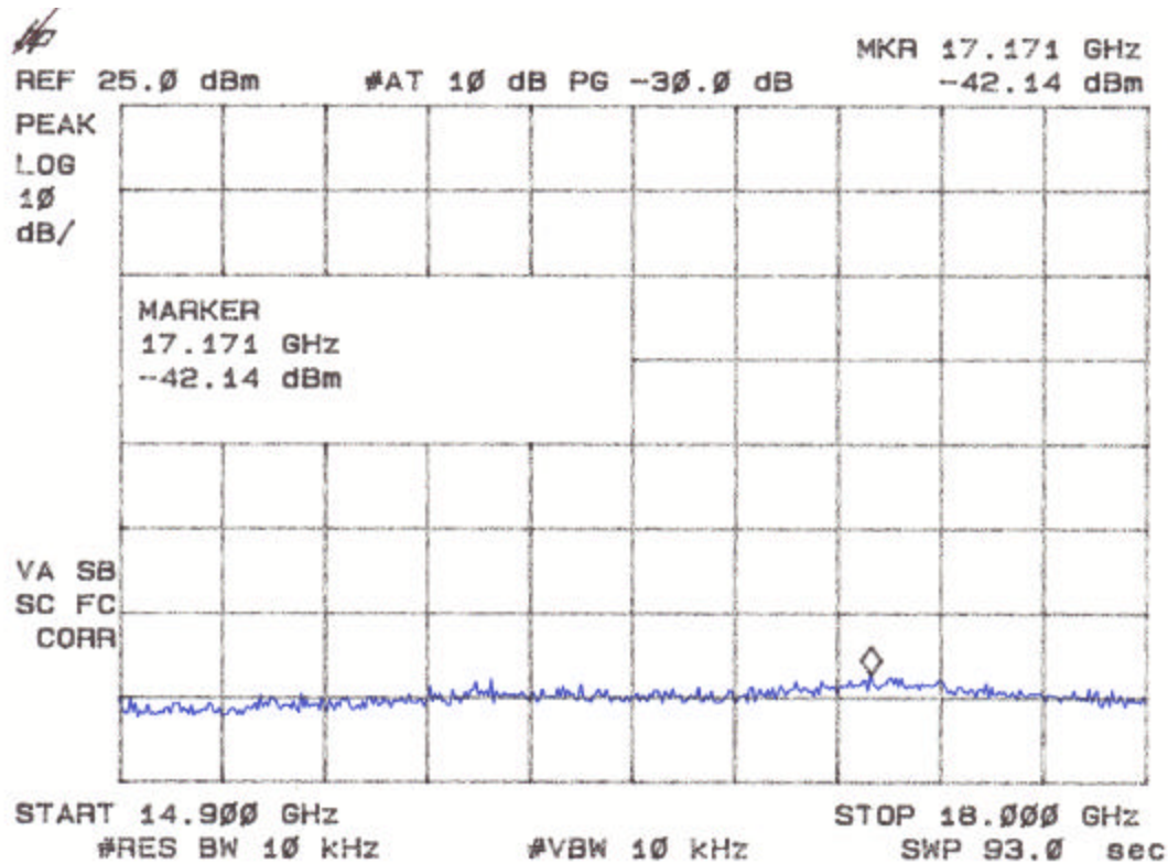
Figure 7g. Spurious Emissions at Antenna Terminals
