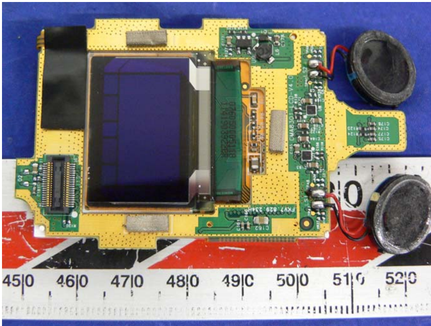
Display Component View 2
