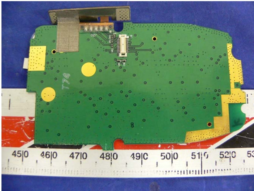
Keyboard Solder View
