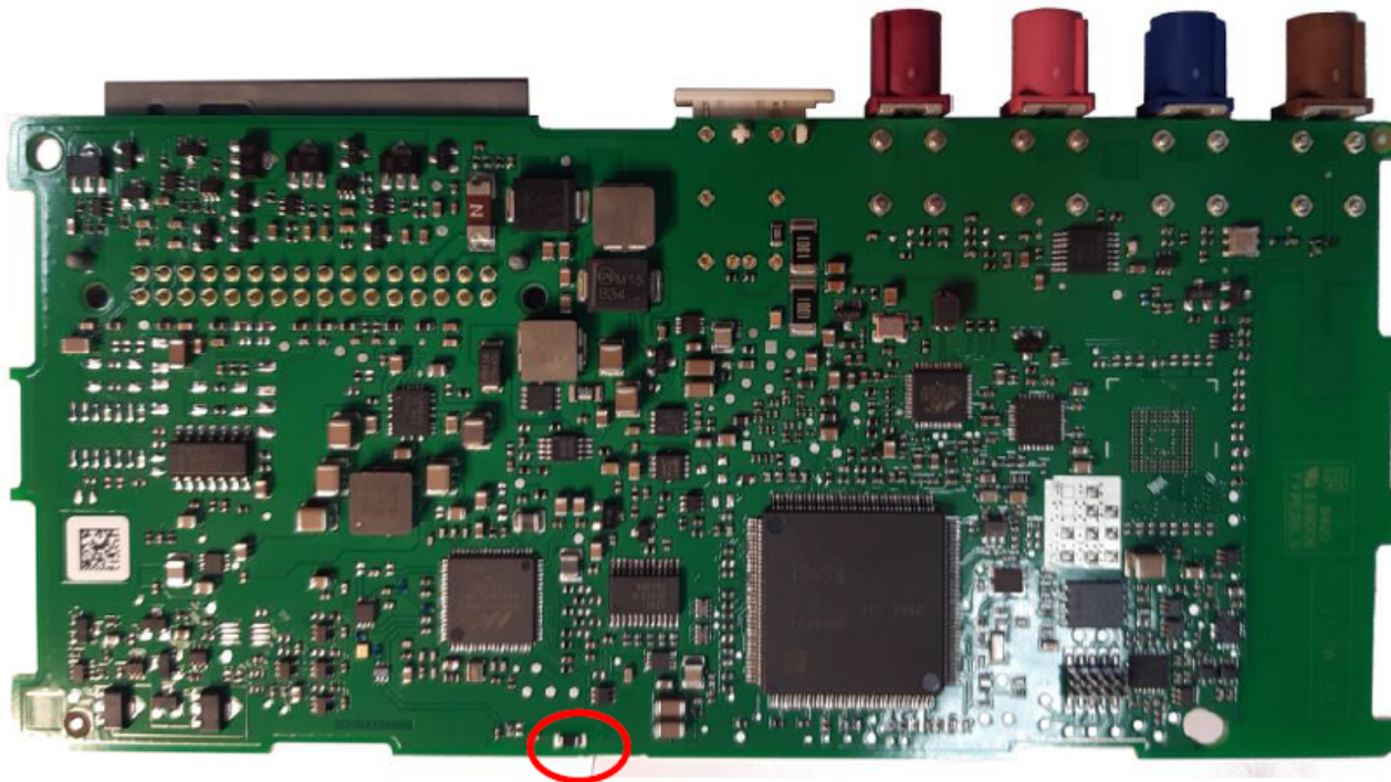
WLAN integrated antenna
