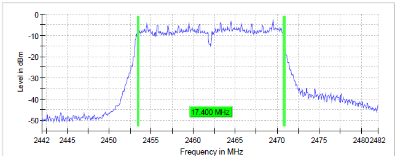
6 dB Bandwidth
