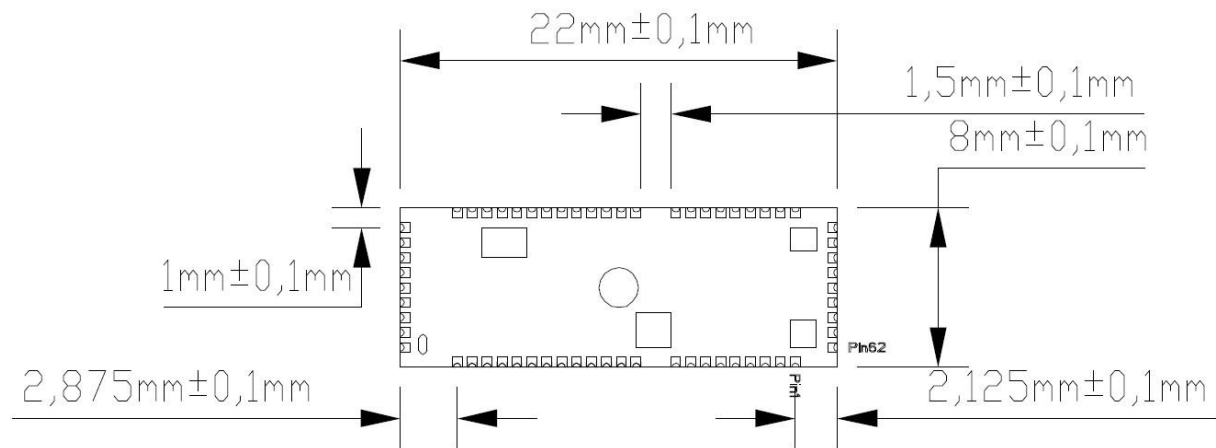
Bottom View
