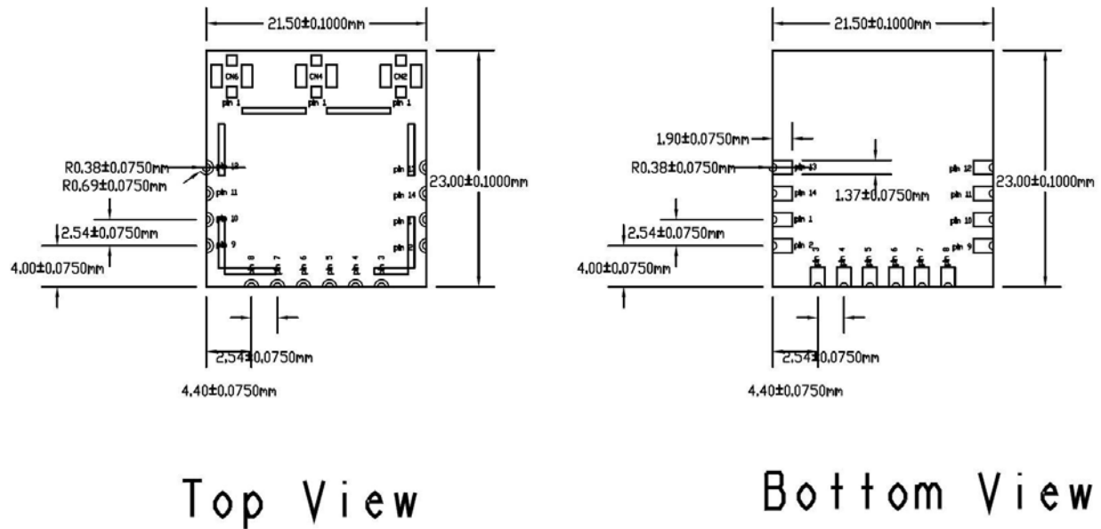
Figure 4 Mechanical Drawing
