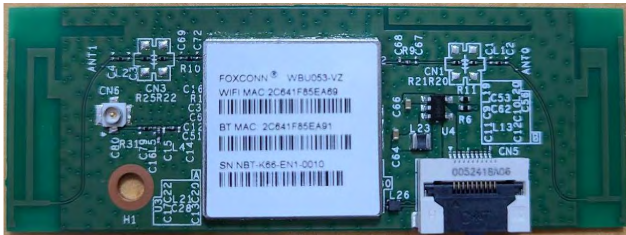
Figure 6 Module Photo (top)
