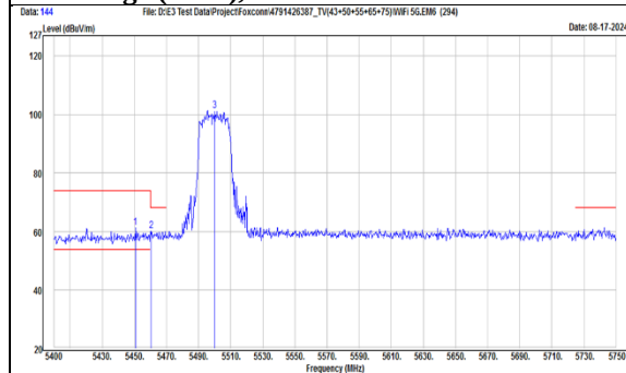
TX, 802.11ax(HE20) (Ch 100) Band Edge (Peak), Horizontal
