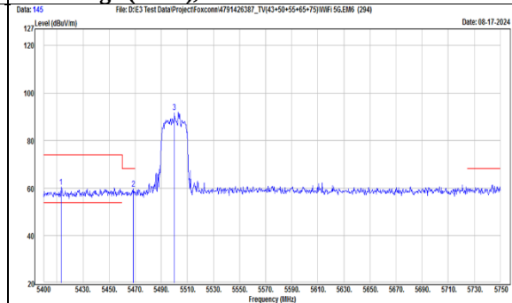
TX, 802.11ax(HE20) (Ch 100) Band Edge (Peak), Vertical
