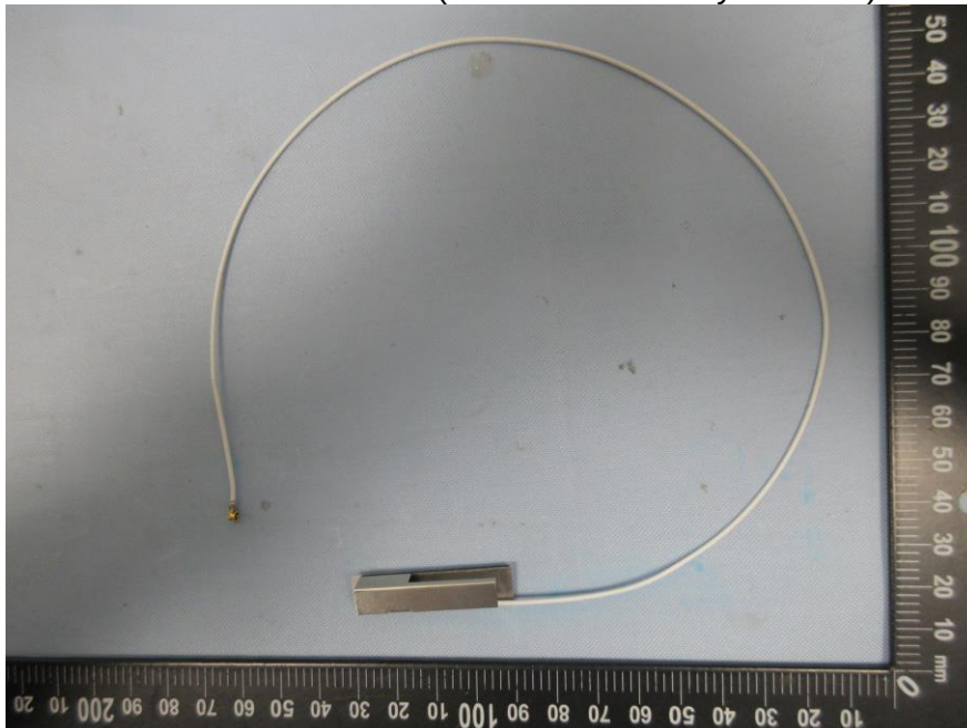
390mm PIFA Antenna (6903B0000P000 by Foxconn)
