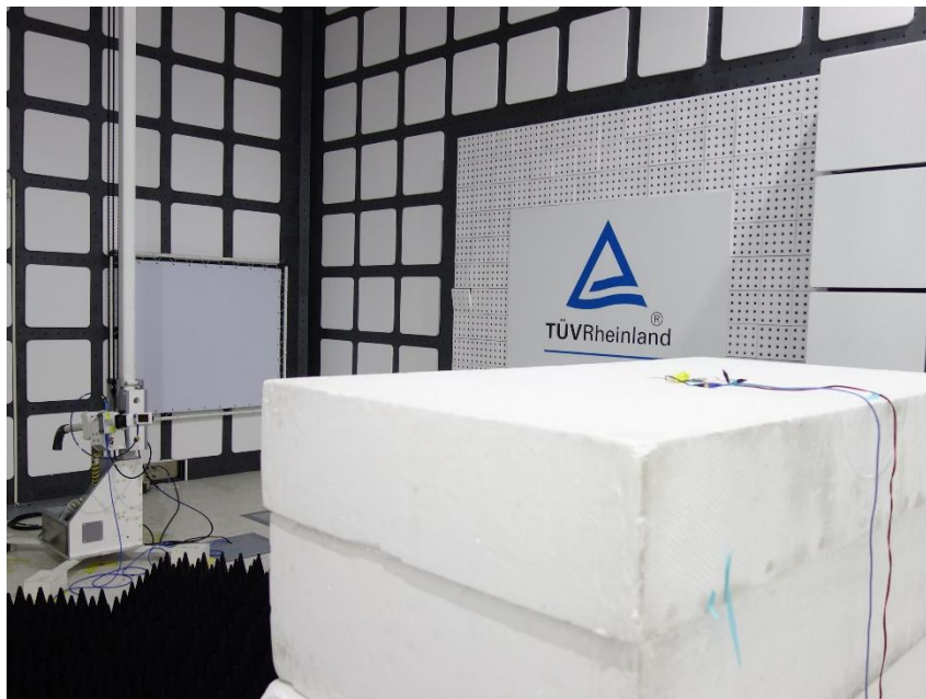
Photograph 6: Test Setup for Spurious Emissions (Back View 4)
