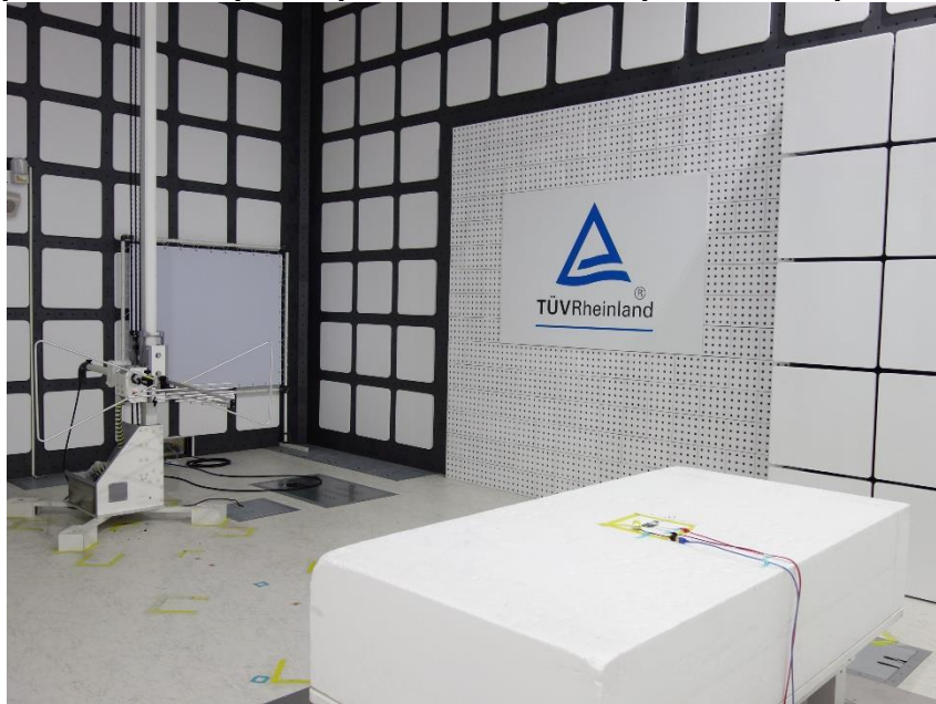
Photograph 4: Test Setup for Spurious Emissions (Back View 2)
