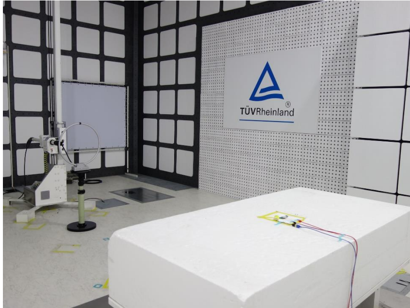
Photograph 3: Test Setup for Spurious Emissions (Back View 1)
