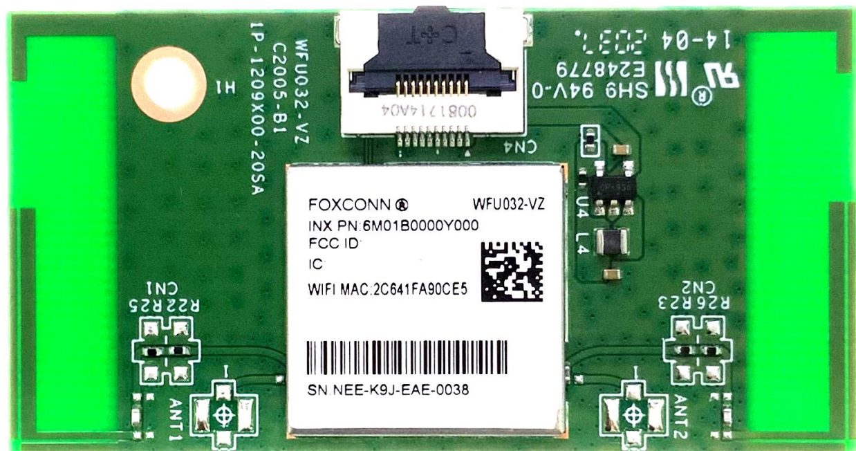
Figure 3 Top Side Photo
