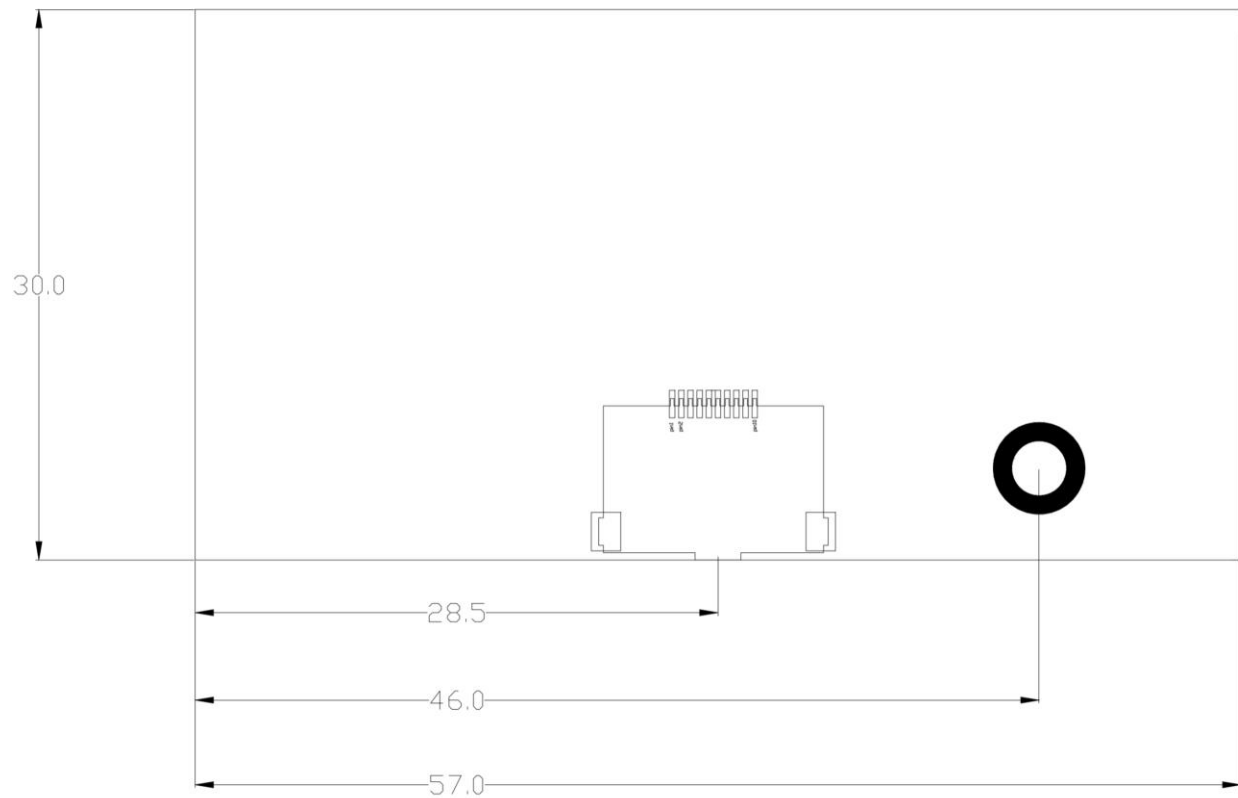
Figure 2 Mechanical Drawing
