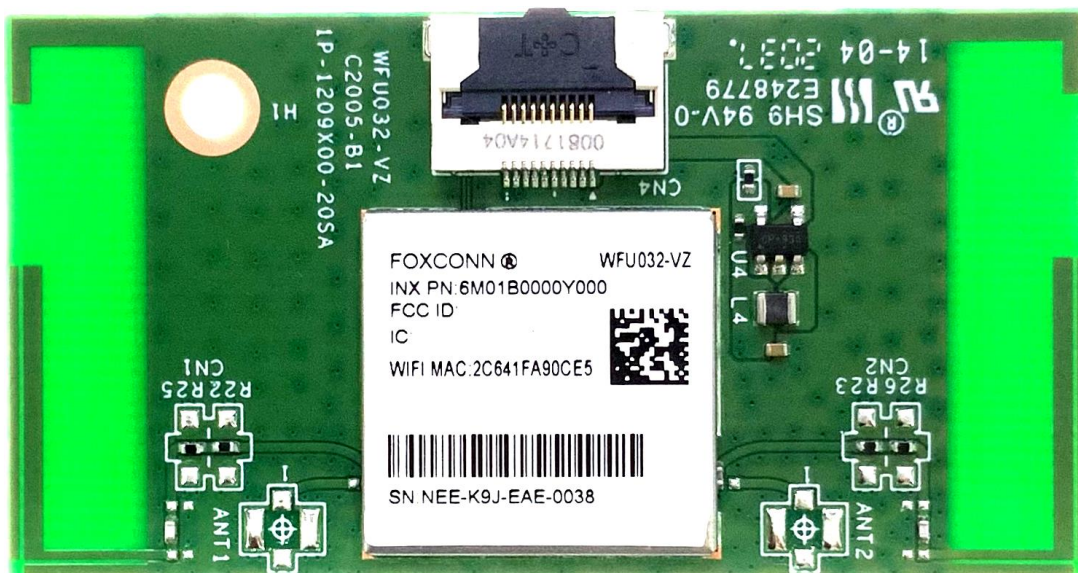
Figure 1 Pin Definitions (Module Top View)
