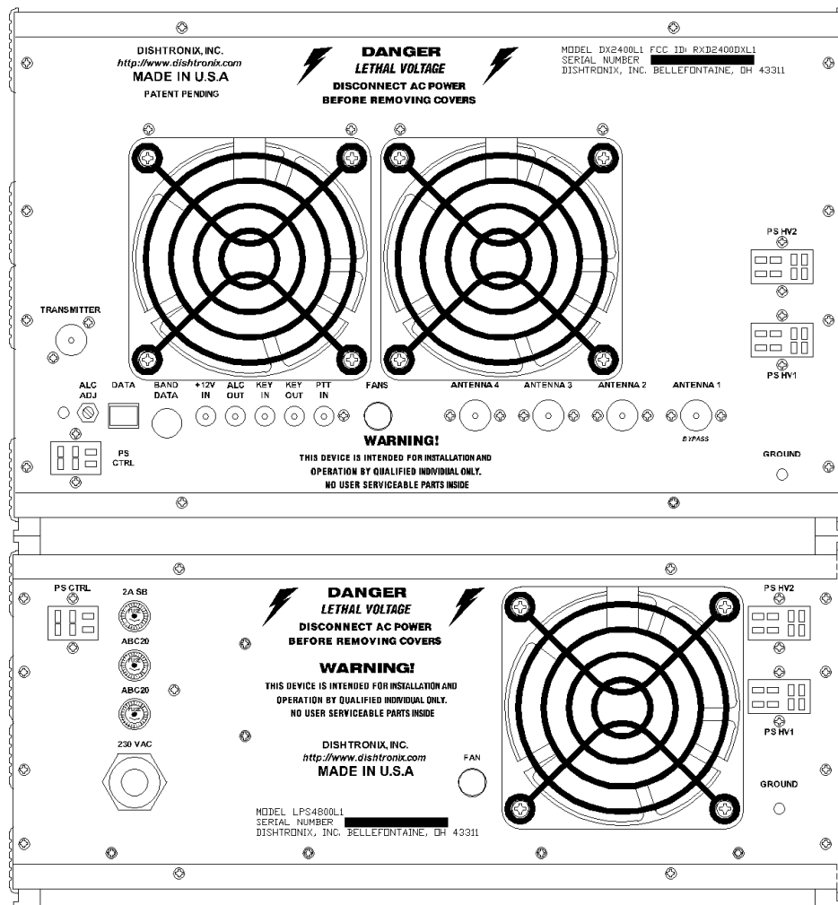
Figure 4. Drawing of DX2400L1 RF Deck (TOP) and LPS4800 Linear Power Supply (Bottom) Rear Panel Silkscreen.
