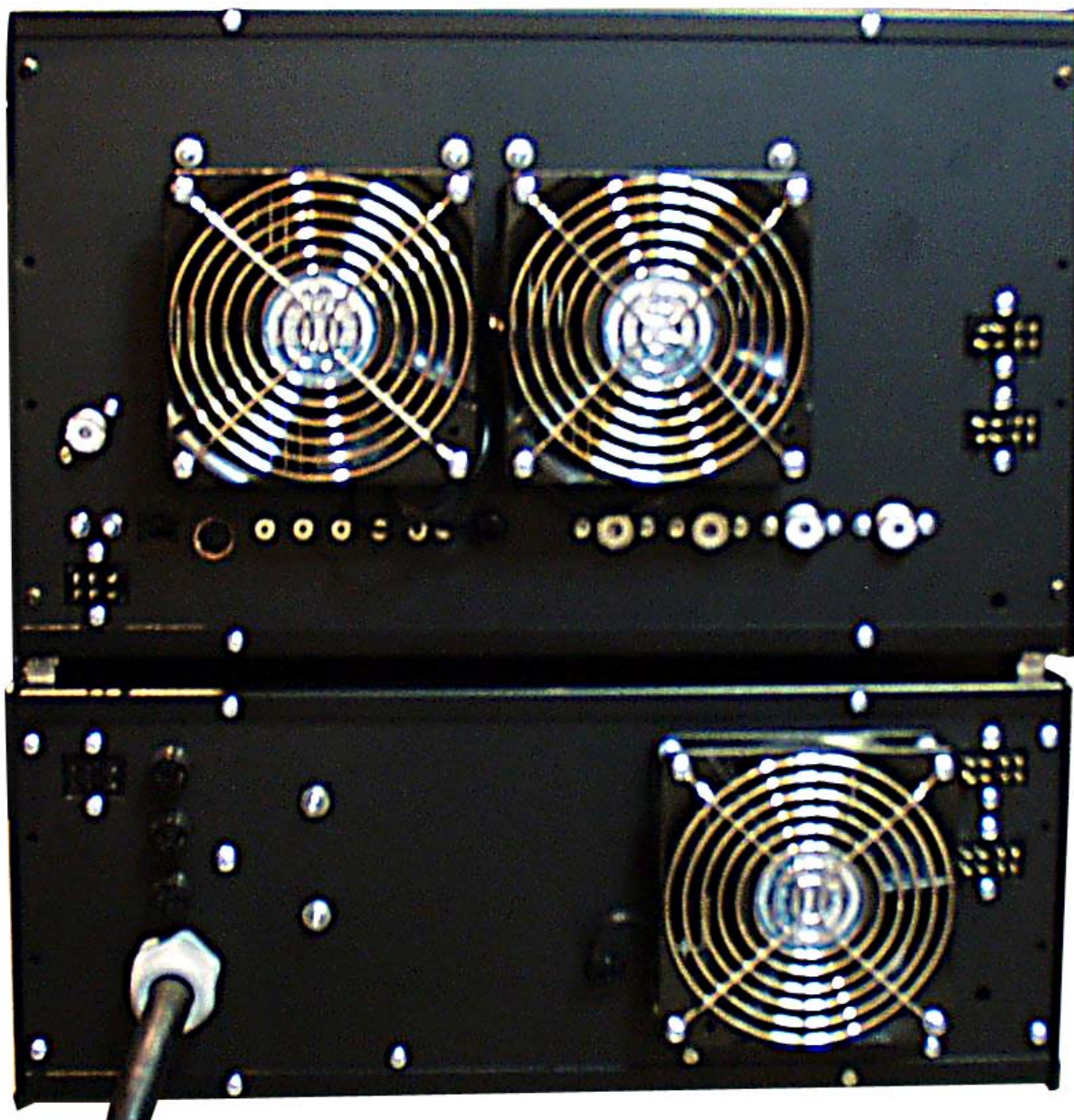
Figure 3. Rear View of DX2400L1 RF Deck (TOP) and LPS4800 Linear Power Supply (Bottom)
