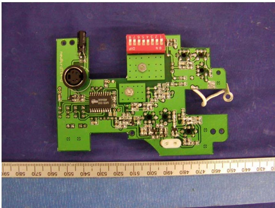
Board 2 – Component View
