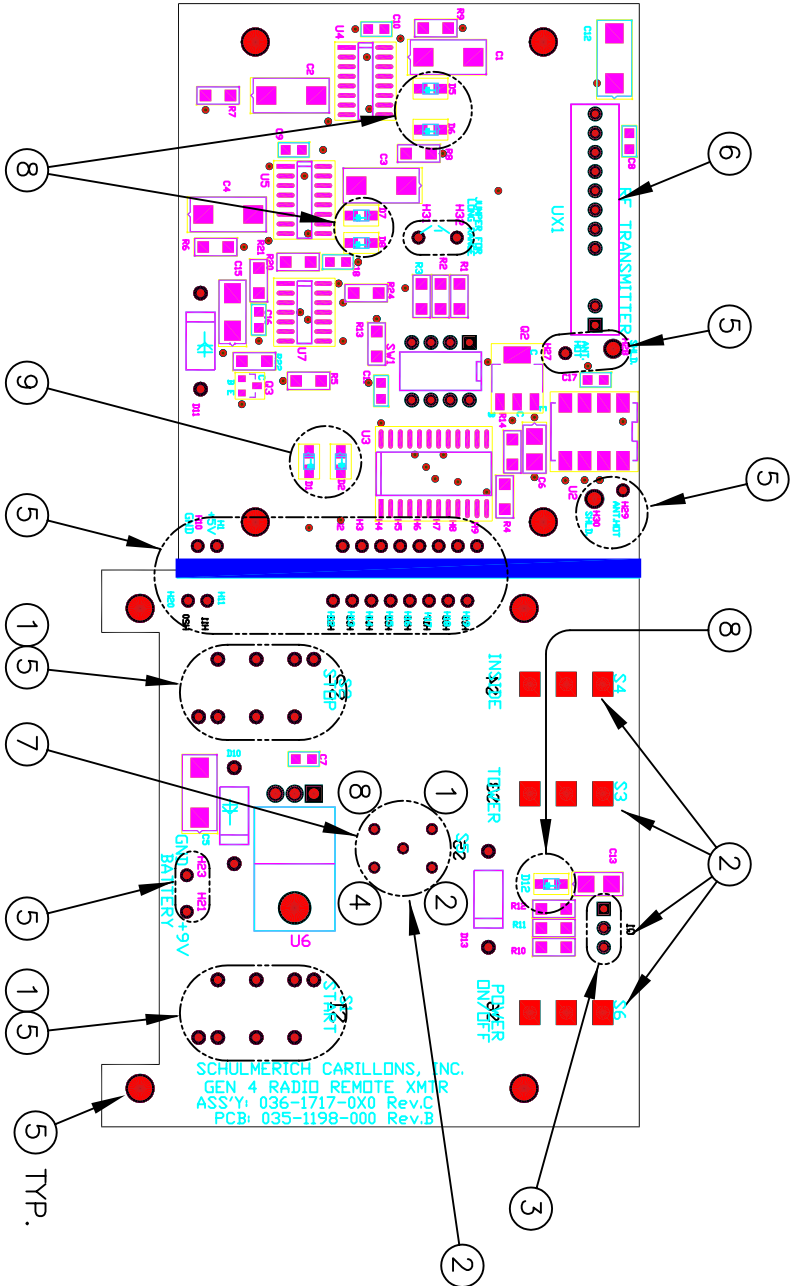
ASSEMBLY TOP
